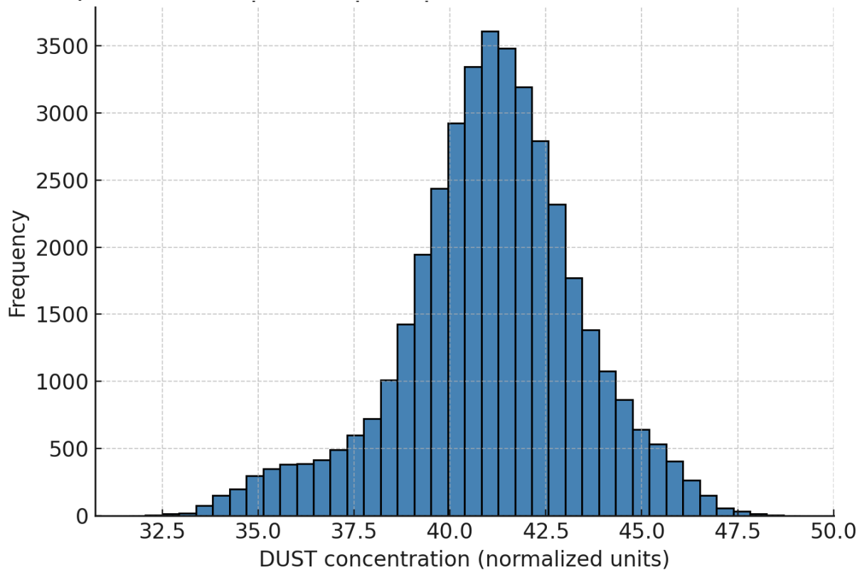
Figure 3. Dust distribution histogram (DUST).
