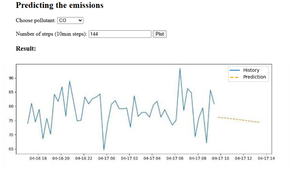
Figure 5. Prediction module interface.
