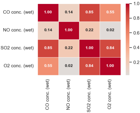
Figure 3. Correlation Between Major Emission Components.
