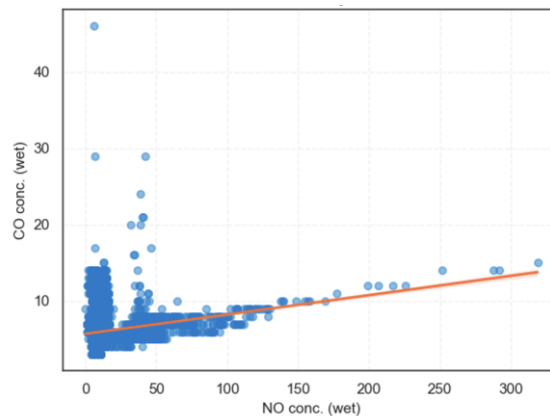
Figure 6. Weak Correlation Between CO and NO Concentrations
