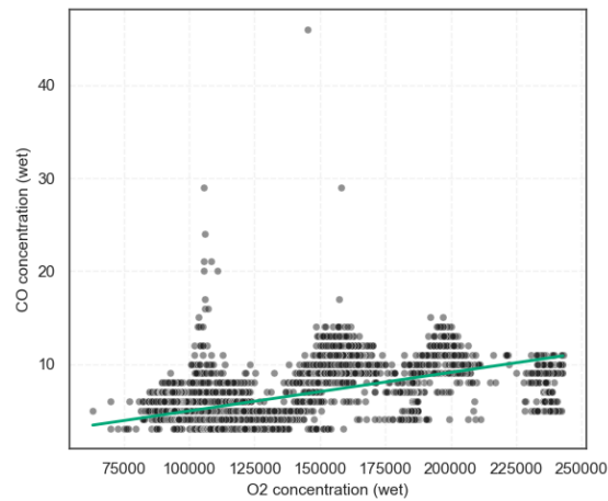
Figure 4. Inverse Relationship Between CO and O 2 Concentrations
