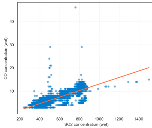
Figure 4. Linear Relationship Between CO and SO 2 Concentrations.
