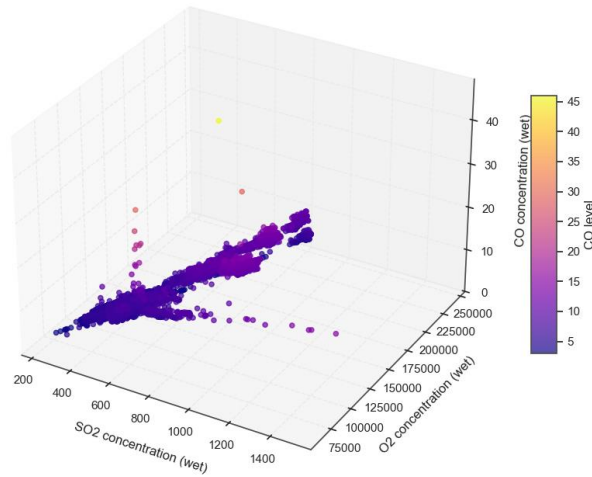
Figure 7. 3D Relationship of CO with SO 2 and O 2 Concentrations.
