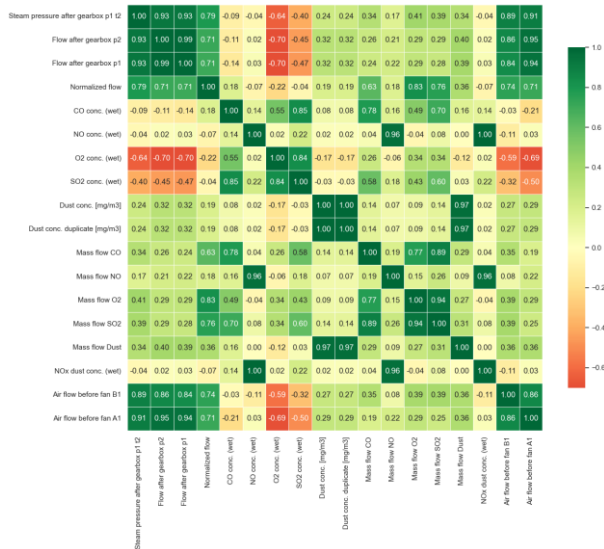
Figure 2. Correlation Matrix of Emission Parameters.
